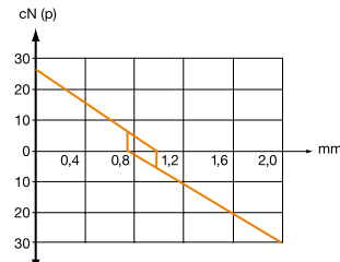
Contact force/travel
